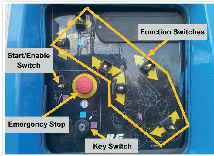
Base control panel JLG
